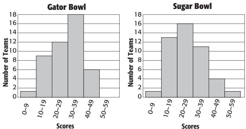
Scores of Winning Teams, 1960–2006
